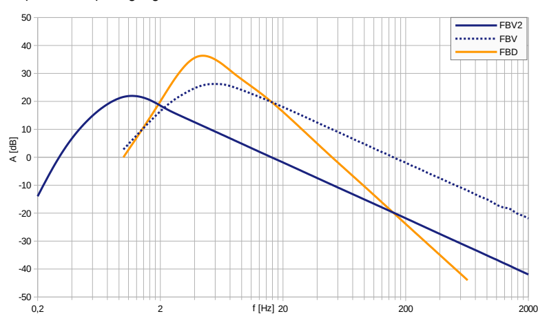
Amplitudenfrequenzgang FBV/FBD
