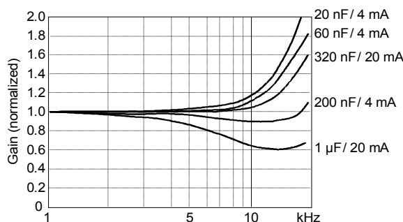
Figure 4: Frequency response of IEPE accelerometers for different cable capacitances and supply currents
