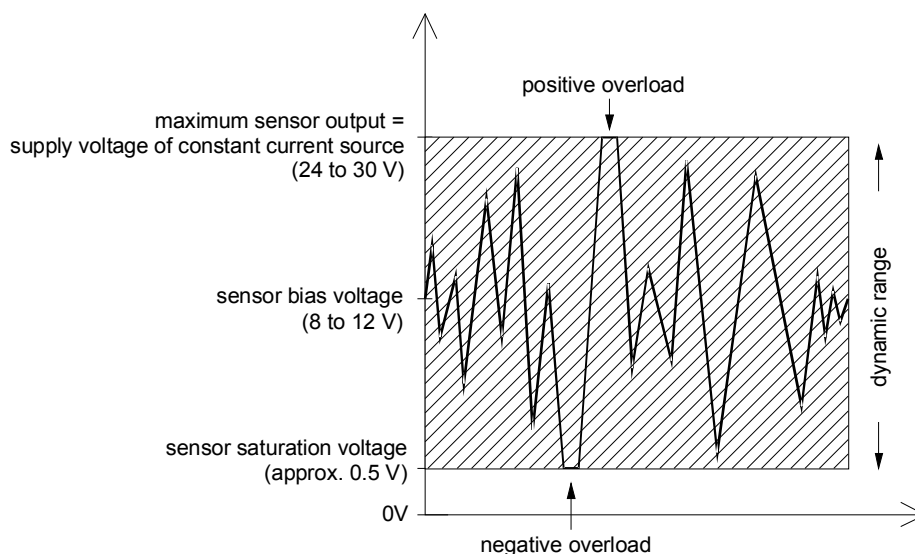
Figure 2: Dynamic range of IEPE transducers
