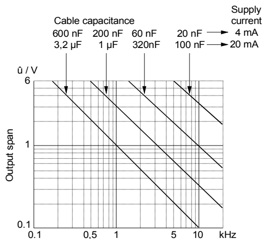
Figure 3: Output span of IEPE accelerometers for different cable capacitances and supply currents
